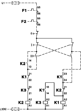
operating with push buttons
