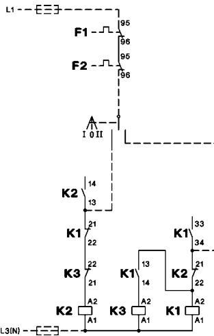
Principal Control Circuit Wiring Diagram operating with control switch
